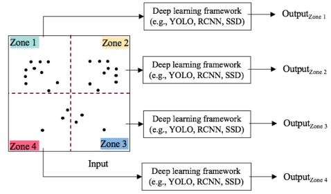
Fig. 4. SVANN-I using fixed-partition-based neighbors. Four distinct models are trained using training samples from each zone.
