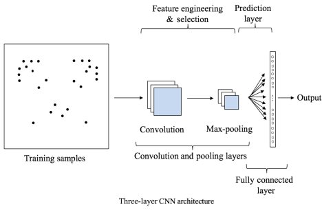
Fig. 3. Spatial OSFA approach using a CNN with three layers: convolution, spatial pooling, and a fully connected layer.
